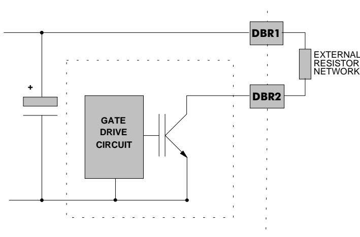
Figure 4.5 Dynamic Braking Circuit
